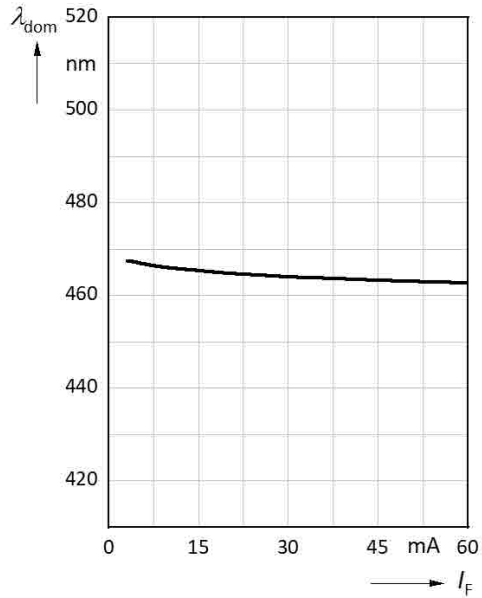
Dominant Wavelength vs. Forward Current
