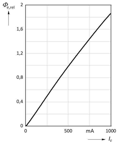
Relative Radiant Flux vs. Forward Current
