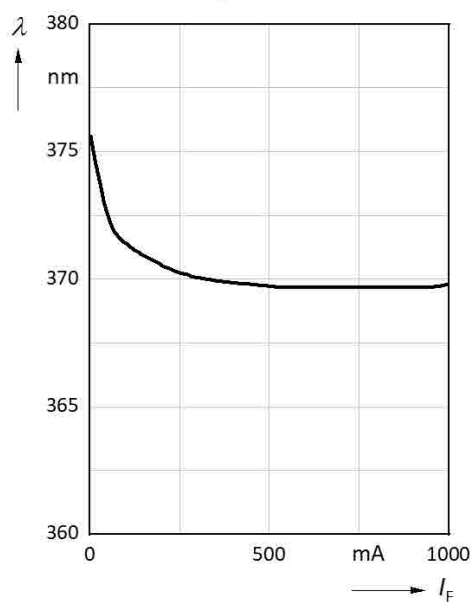
Peak Wavelength vs. Forward Current
