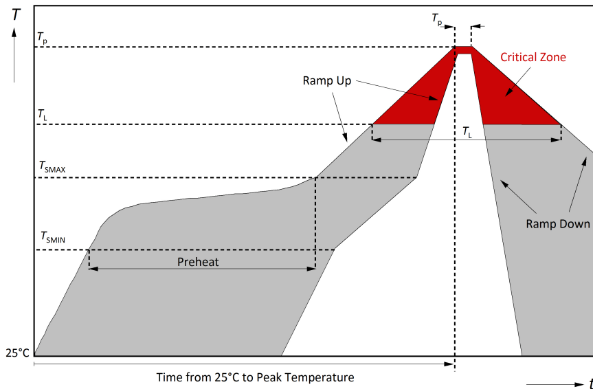
Soldering Profile (Temperature vs. Time)
